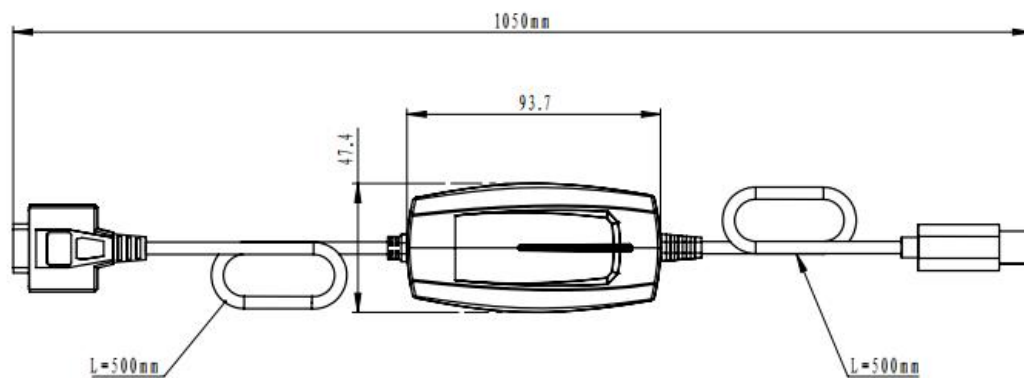
Figure 1-1 Mechanical Dimensions
