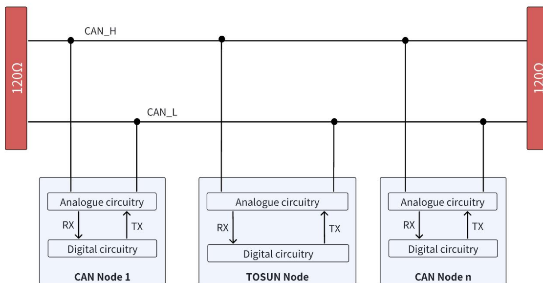
Figure 2-2 Connect to CAN Bus
