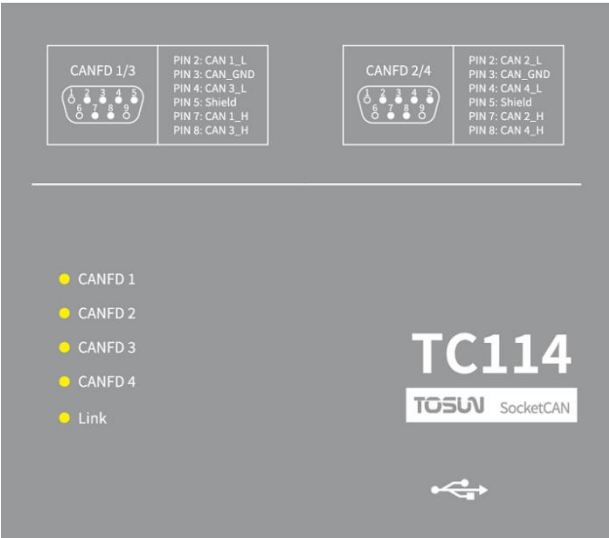
Figure 1-2 Front Panel Layout
