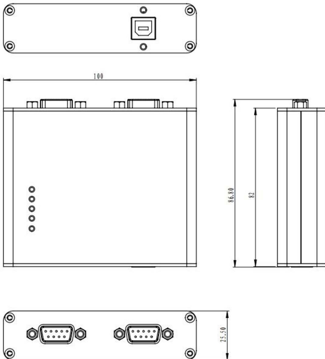
Figure 1-1 Mechanical Dimensions
