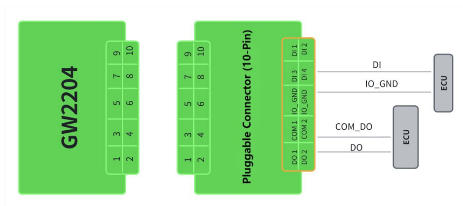
Figure 2-8 Pluggable Connector (10-Pin) for I/O
