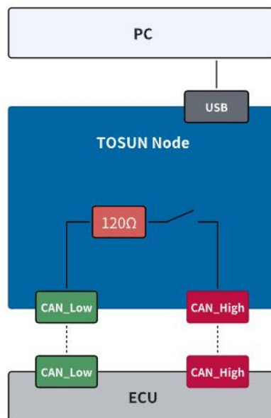
Figure 2-6 Using CAN
