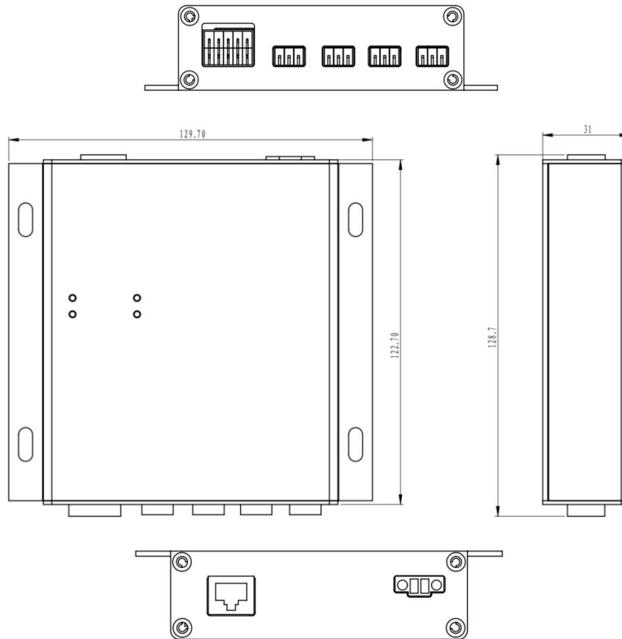
Figure 1-1 Mechanical Dimensions
