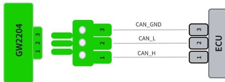
Figure 2-5 3-Pin Pluggable Terminal (CAN)
